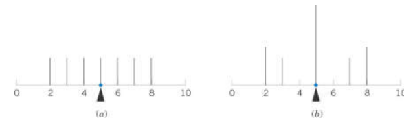
Figure 3-6 These probability distributions have the same mean and variance measures, but are very different in shape.
