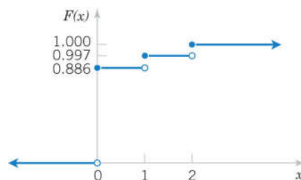
Figure 3-4 CDF. Note that F(x) is defined for all x , -\infty < x < \infty , not just 0, 1 and 2.
