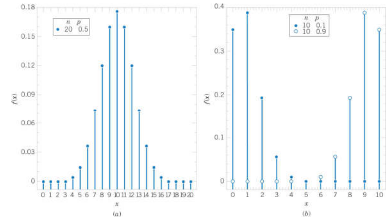
Figure 3-8 Binomial Distributions for selected values of n and p . Distribution (a) is symmetrical, while distributions (b) are skewed. The skew is right if p is small.
