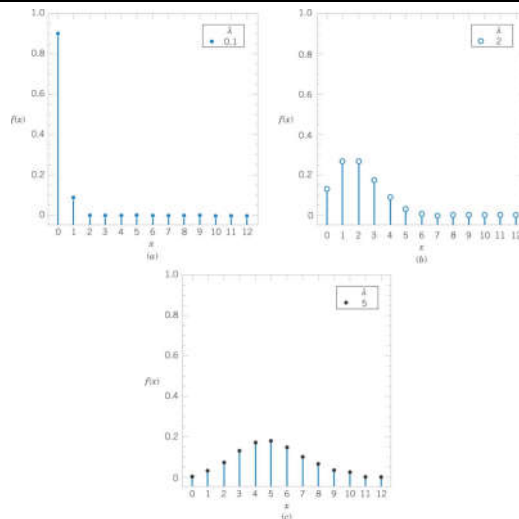
Figure 3-14 Poisson distributions for \lambda = 0.1, 2, 5 .
