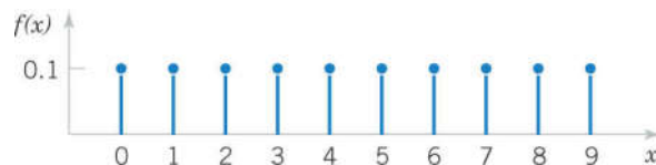
Figure 3-7 Probability mass function, f(x) = 1/10 for x = 0, 1, 2, \dots, 9
