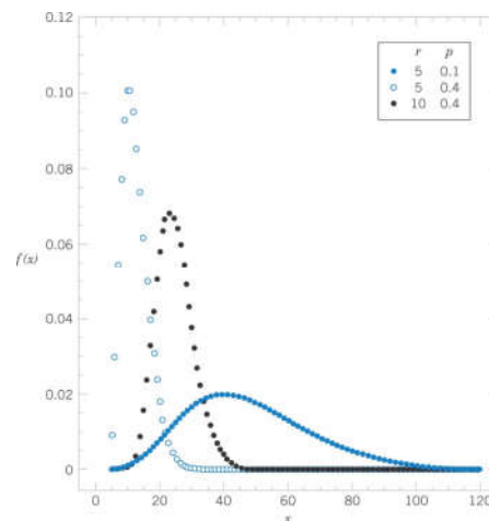
Figure 3-10 Negative binomial distributions for 3 different parameter combinations.
