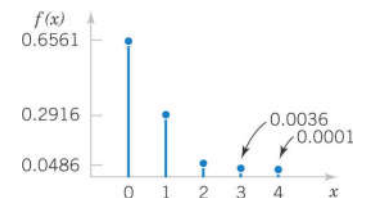
Figure 3-1 Probability distribution for bits in error.
