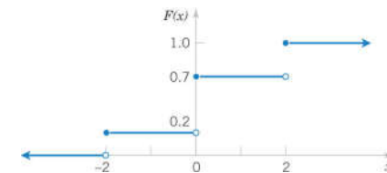
Figure 3-3 Graph of the CDF
